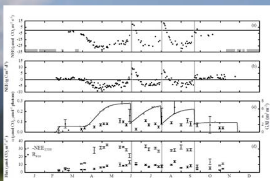
Fig. 2 Seasonal course of various NEE metrics and GAI.
