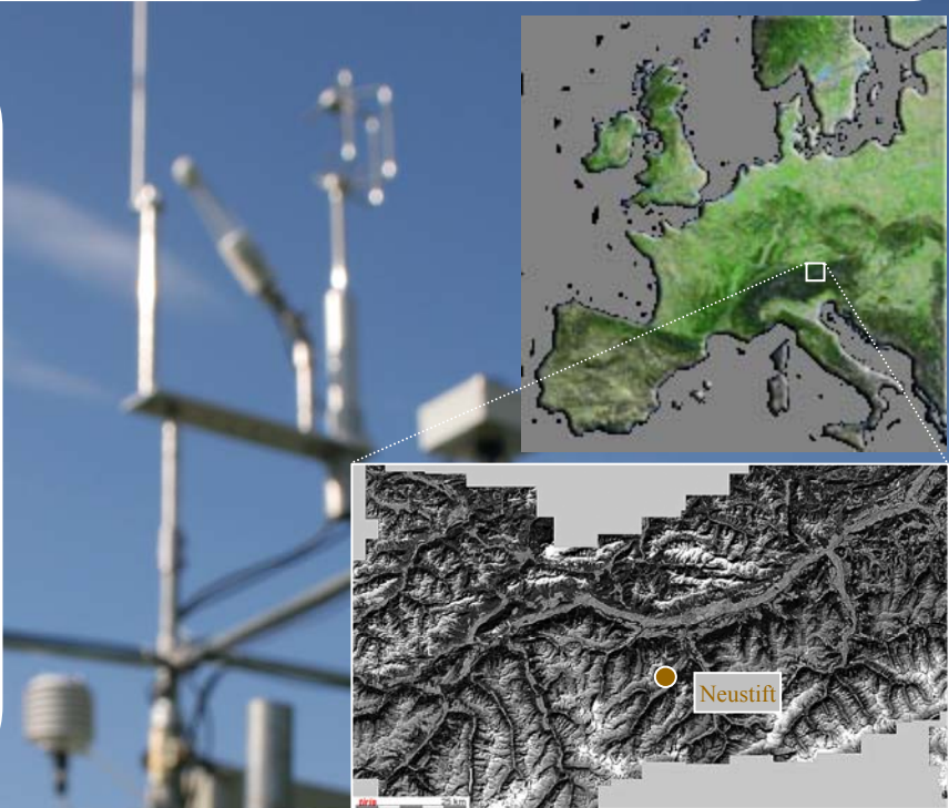
Figure 1 Location of study sites in Tyrol, Austria.
