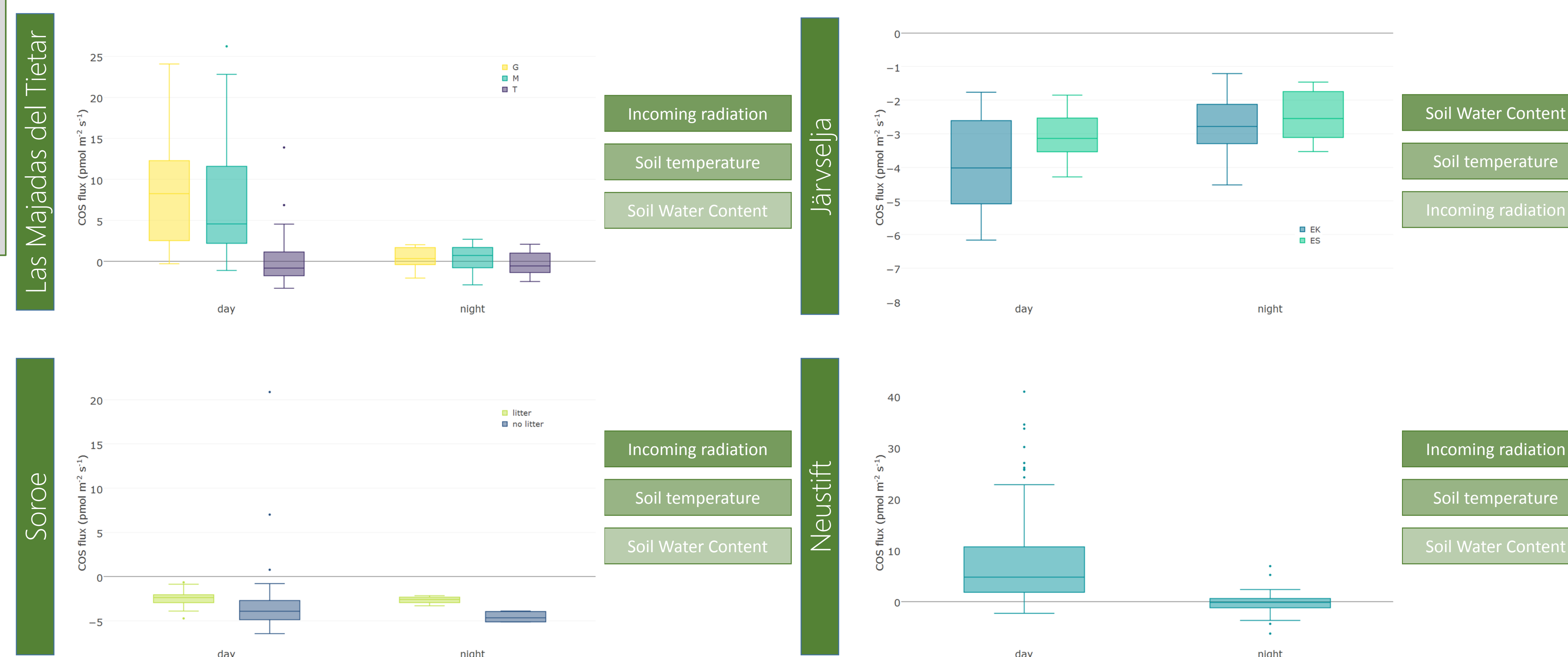
(IV) Boxplots summarizing the soil chamber measurements in Las Majadas, Soroe, Järvelja and Neustift. Night-(zenith above 90°) and daytime measurements are displayed separately. In Las Majadas (Spain) measurements were taken under Trees (T), in the open savannah (G) and inbetween (M). In Soroe (Denmark) some soil-rings were freed from litter (no litter), the rest kept their natural amount of litter (litter). In Järvelja (Estonia) some rings were placed on elevated spots (EK) and some in depressions (ES). Next to the boxplots a ranking of the predictors (random forest regression) for the COS soil flux – starting from most important to least important.
