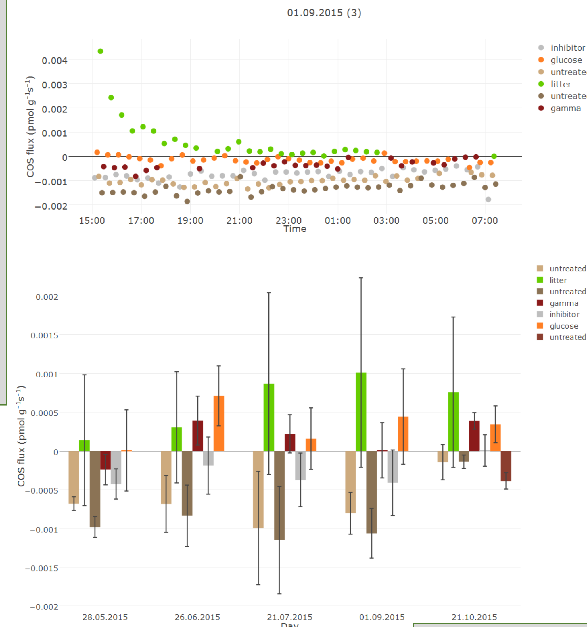
(IV) COS fluxes from the different treatments; COS emission from the litter treatment started high and decreased fast over the course of the measurement. This pattern can be seen on all days (not shown). Untreated soil samples exhibited COS uptake, which decreased, when the CA inhibitor was added or the samples were sterilized (gamma).
